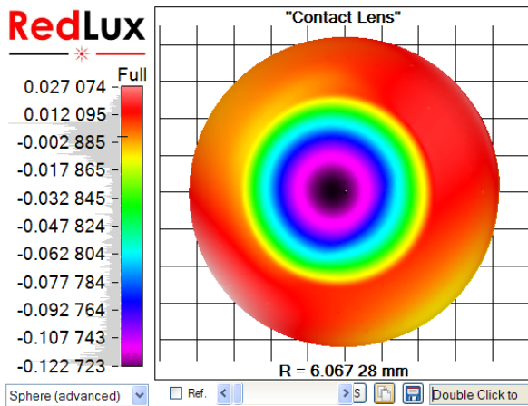
Figure 1: Form of the front surface, taking the outer section as reference.
