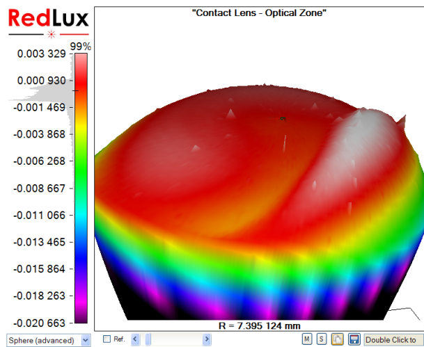
Figure 4: Detail view of optical zone. The deviation from the best-fit sphere has been magnified to show topography.
